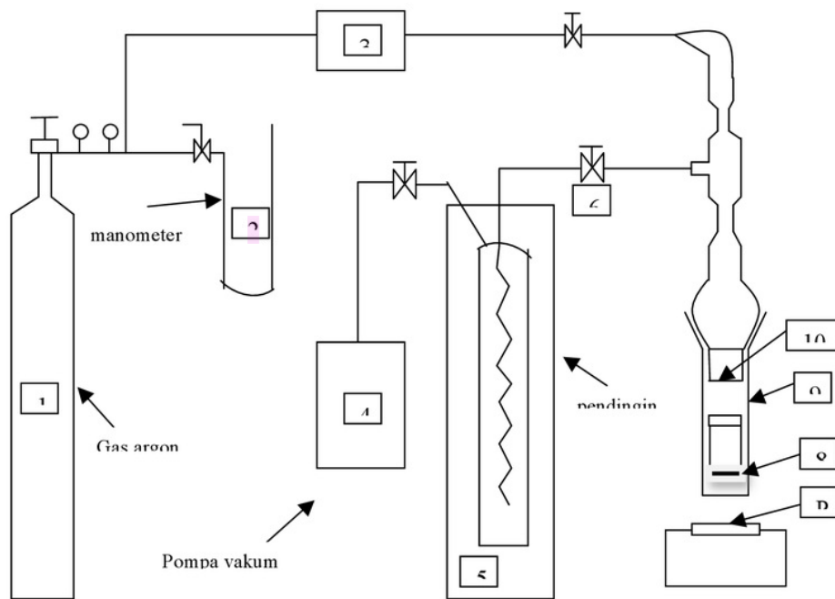
Gambar 2. Skema Alat Close Space Vapour Transport ( CSVT)
